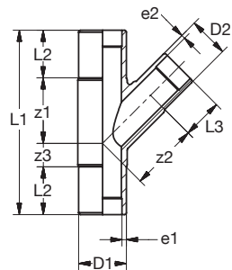
BR PE100 Abzweig 45° red lang SDR17(-11) schwarz BR PE100 Branch 45° red long SDR17(-11) black
