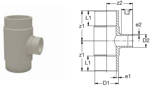
BR PP-INDUSTRIAL T-Stück 90° red kurz st SDR11 grau BR PP-INDUSTRIAL Tee 90° red short butt SDR11 grey
