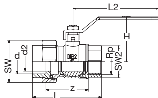
BR PP-RCT Ü-Kugelhahn-Messing IG-zyl verschraubt Runddichtring-EPDM grün BR PP-RCT Transition-Ball valve Brass female-thread-cyl with union-nuts O-Ring-gasket-EPDM green
