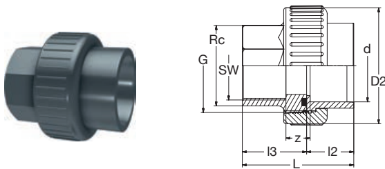
BR PVC-U Ü-Verschraubung IG-keg Runddichtring-EPDM grau BR PVC-U Transition-Union female-thread-con O-Ring-gasket-EPDM grey
