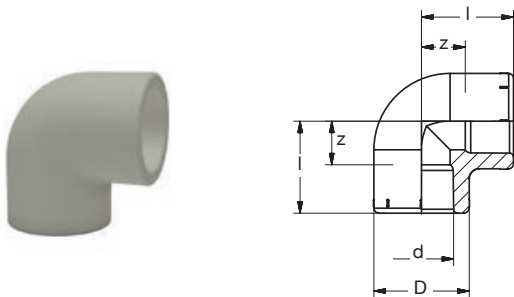
BR PP-INDUSTRIAL Winkel 90° grau
